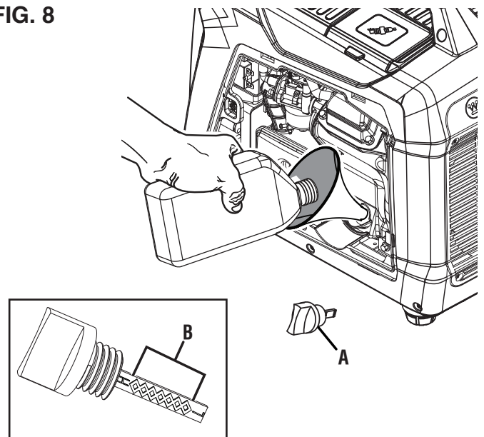
A - Oil Dipstick B - Safe Operating Range
