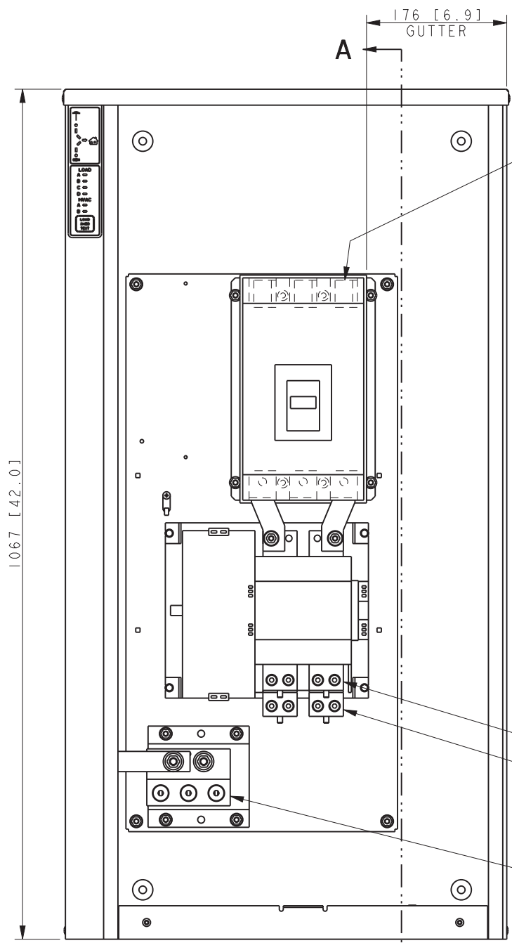
300-400A INNER PANEL & COVER REMOVED TO SHOW DETAIL
