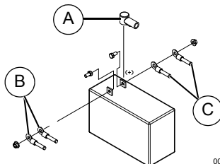
Figure 4-5. Battery Connection
