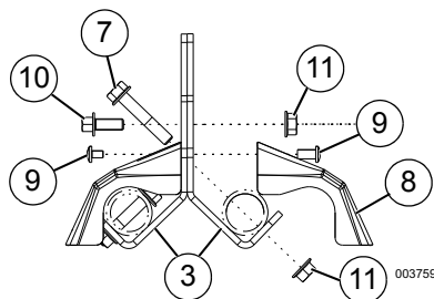
Figure 2-9. Steel Lifting Pocket Assembly
