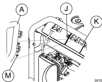
Figure 2-10. Handle Assembly
