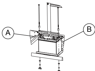
Figure 4-5. Battery Connection
