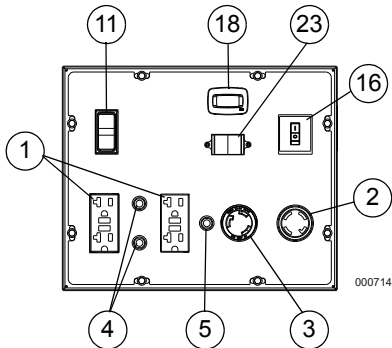
Figure 2-2. Control Panel
