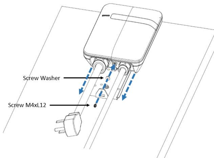
Figure 2-4 Screw locking position
