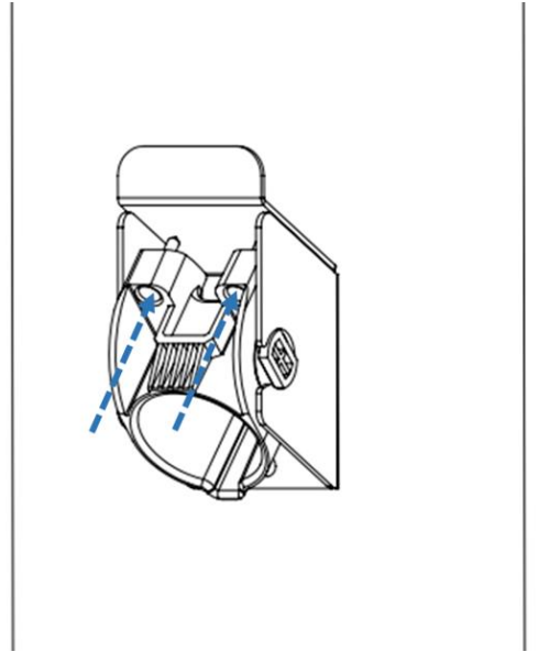
Figure 2-12 Lock screws
