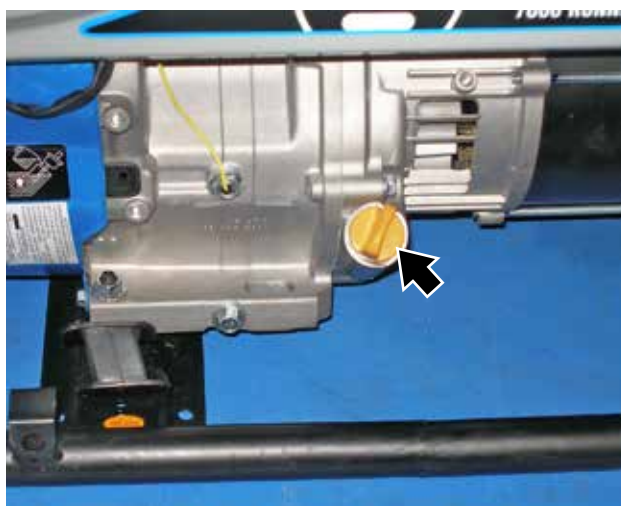
Figure 26 – Oil Fill Plug/Dipstick
