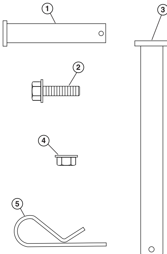
Figure 3 – Wheel Kit Hardware
