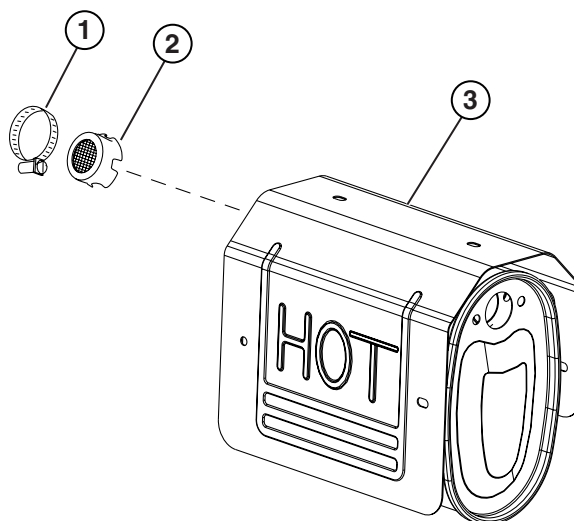
Figure 42 – Spark Arrestor Assembly
