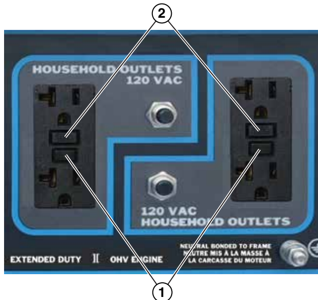
Figure 39 – GFCI Outlet
