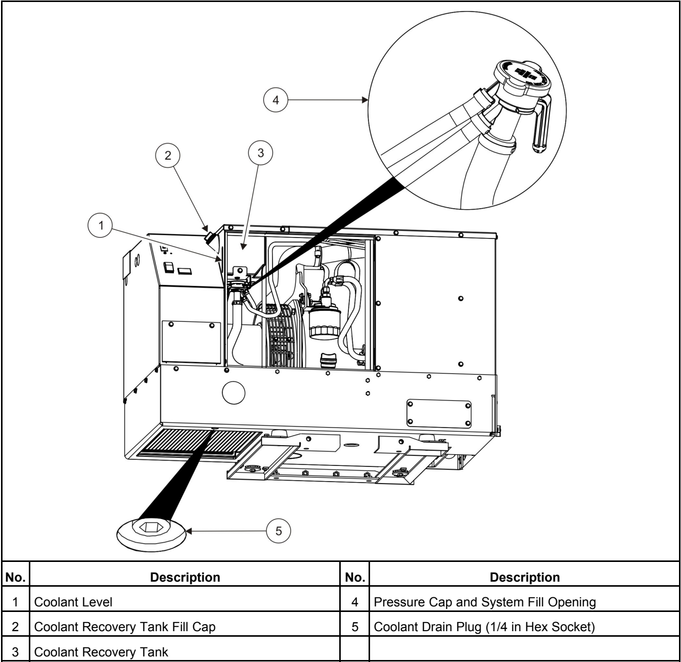
FIGURE 9. COOLING SYSTEM
